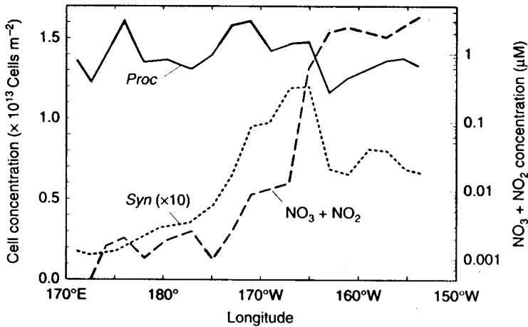
Figure 1. Integrated concentrations of Prochlorococcus and Synechococcus and concentration of nitrate and nitrite in surface, along a transect in the equatorial Pacific between the warm pool (165°E) and HNLC waters (150°W). Data were collected during the FLUPAC cruise, held during fall 1994 (Blanchot, unpublished data; nutrient data are from Eldin et al. 1997).
