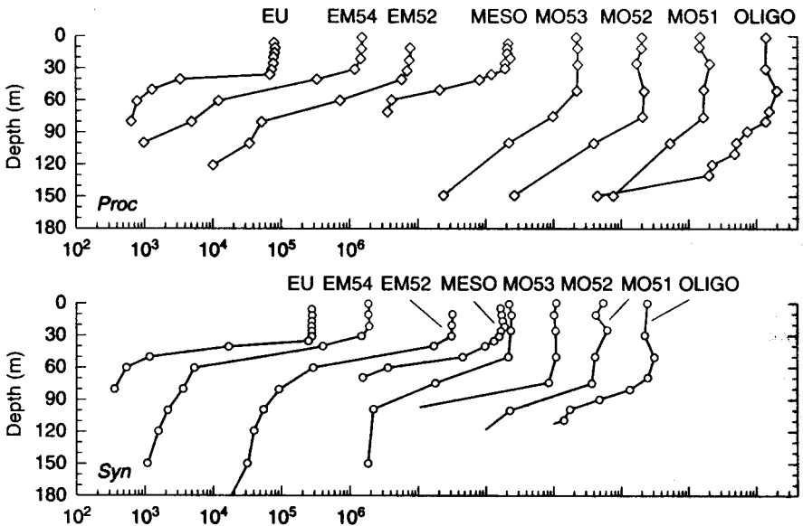
Figure 2. Vertical profiles of Prochlorococcus ( Proc ) and Synechococcus ( Syn ) cell concentrations along the transect from the EU (20°32'N 18°34'W) to OLIGO site (21°02'N 31°08'W) during December 1992 (EUMELI 5). For each profile, the abscissa ranges from 10^2 to 10^6 cells \text{ml}^{-1} , but consecutive profiles are shifted by one decade. Modified from Partensky et al. (1996) with permission.
