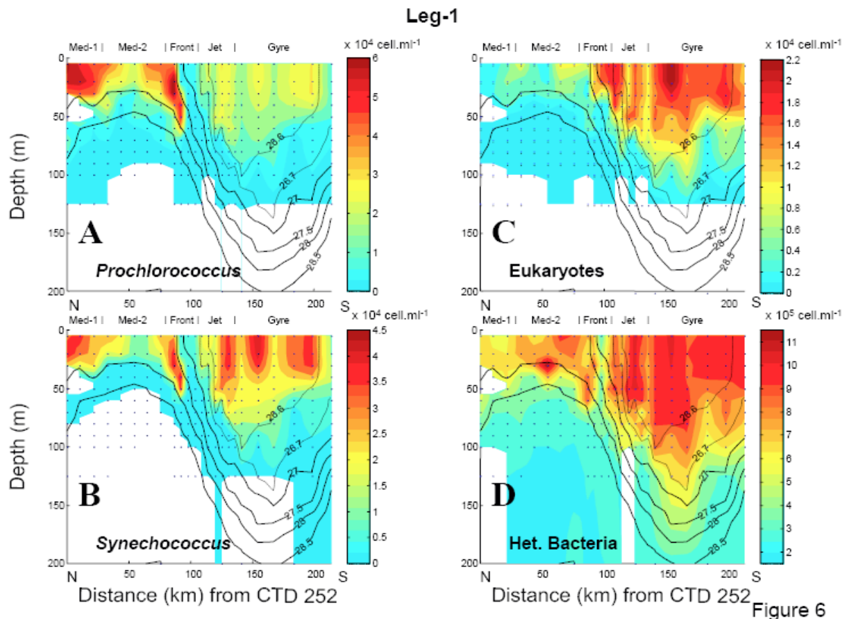
Figure 6 : Distribution of picoplanktonic populations along the transect 2 of leg-1 of the Almofront-2 cruise. (A) Prochlorococcus , (B) Synechococcus , (C) picoeukaryotes, (D) heterotrophic bacteria. Distances are given in km from CTD 252 (North). Density isolines are expressed in \text{kg.m}^{-3} . Note that the color scale varies with groups.
